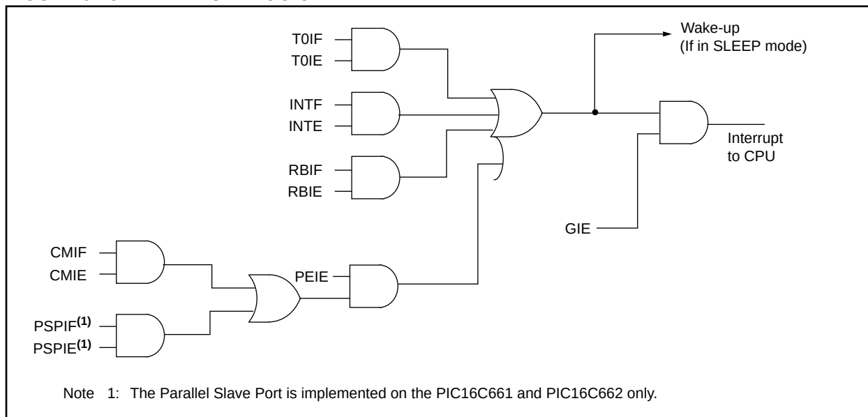
FIGURE 9-15: INTERRUPT LOGIC
