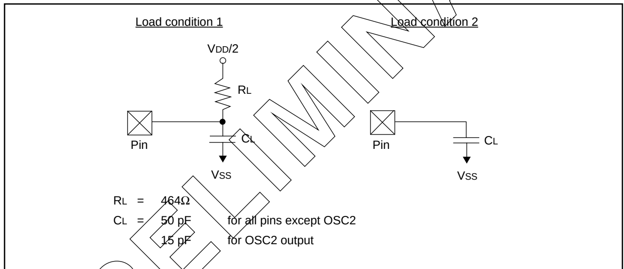
FIGURE 12-1: LOAD CONDITIONS
