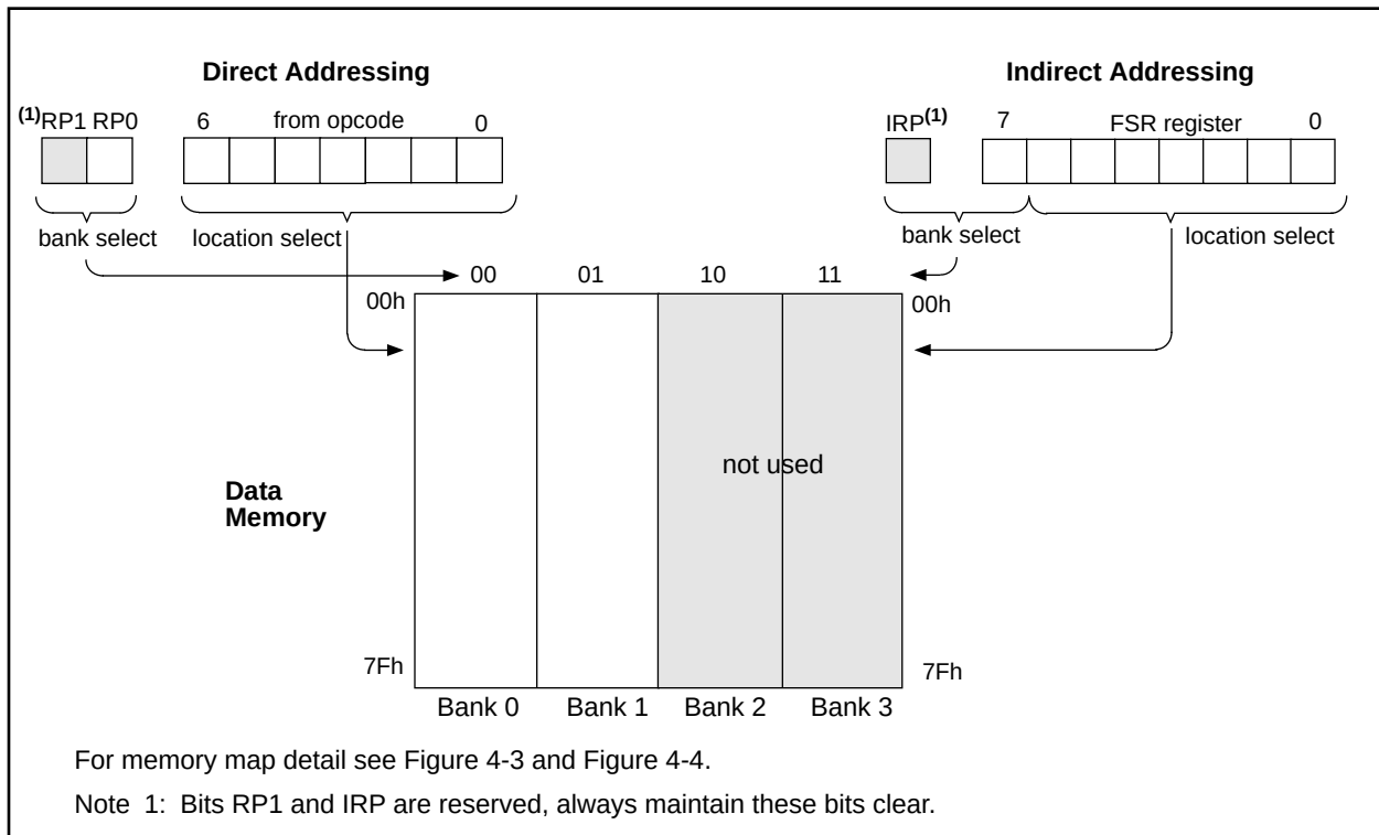
FIGURE 4-12: DIRECT/INDIRECT ADDRESSING
