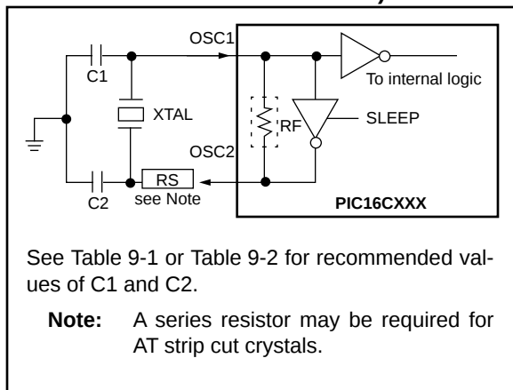
FIGURE 9-2: CRYSTAL OPERATION (OR CERAMIC RESONATOR) (HS, XT OR LP OSC CONFIGURATION)
