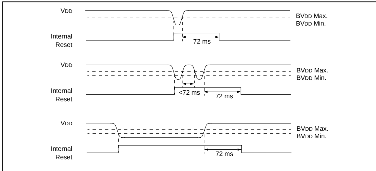
FIGURE 9-8: BROWN-OUT SITUATIONS
