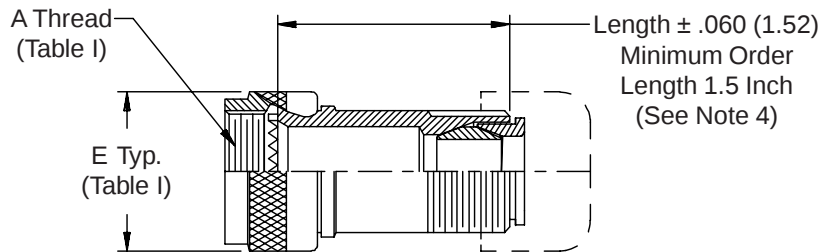
Anti-Rotation Device (Typ.)
