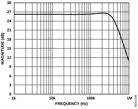
Figure 6. Typical Small-Signal Bandwidth ( V_{OUT} = 200\text{ mV p-p} )
