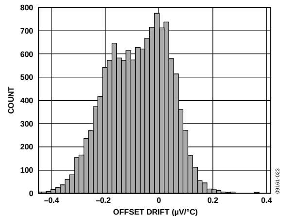
Figure 23. Input Offset Drift Distribution
