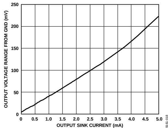
Figure 18. Output Voltage Range From GND vs. Output Sink Current
