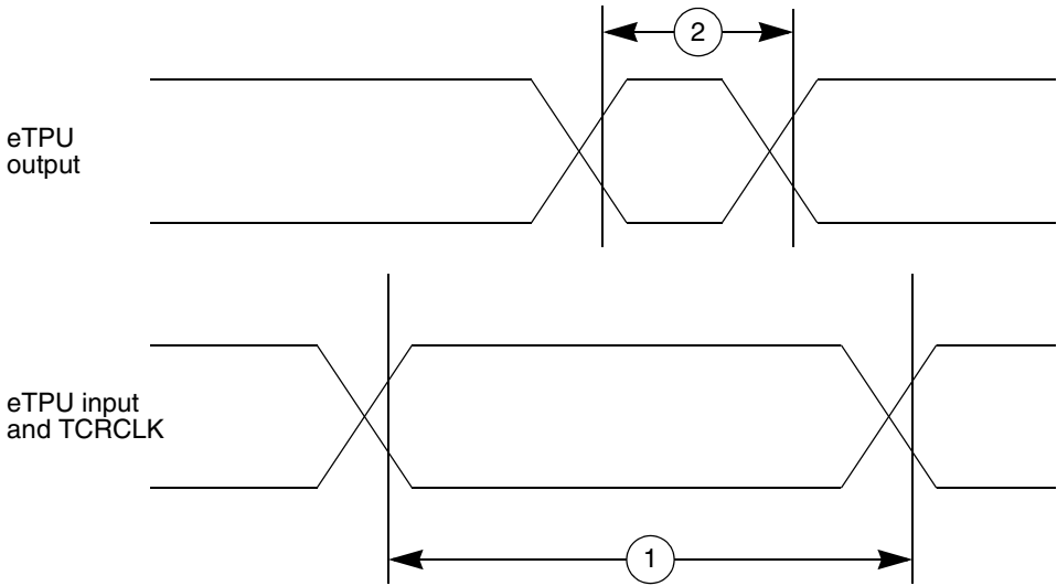
Figure 16. eTPU Timing
