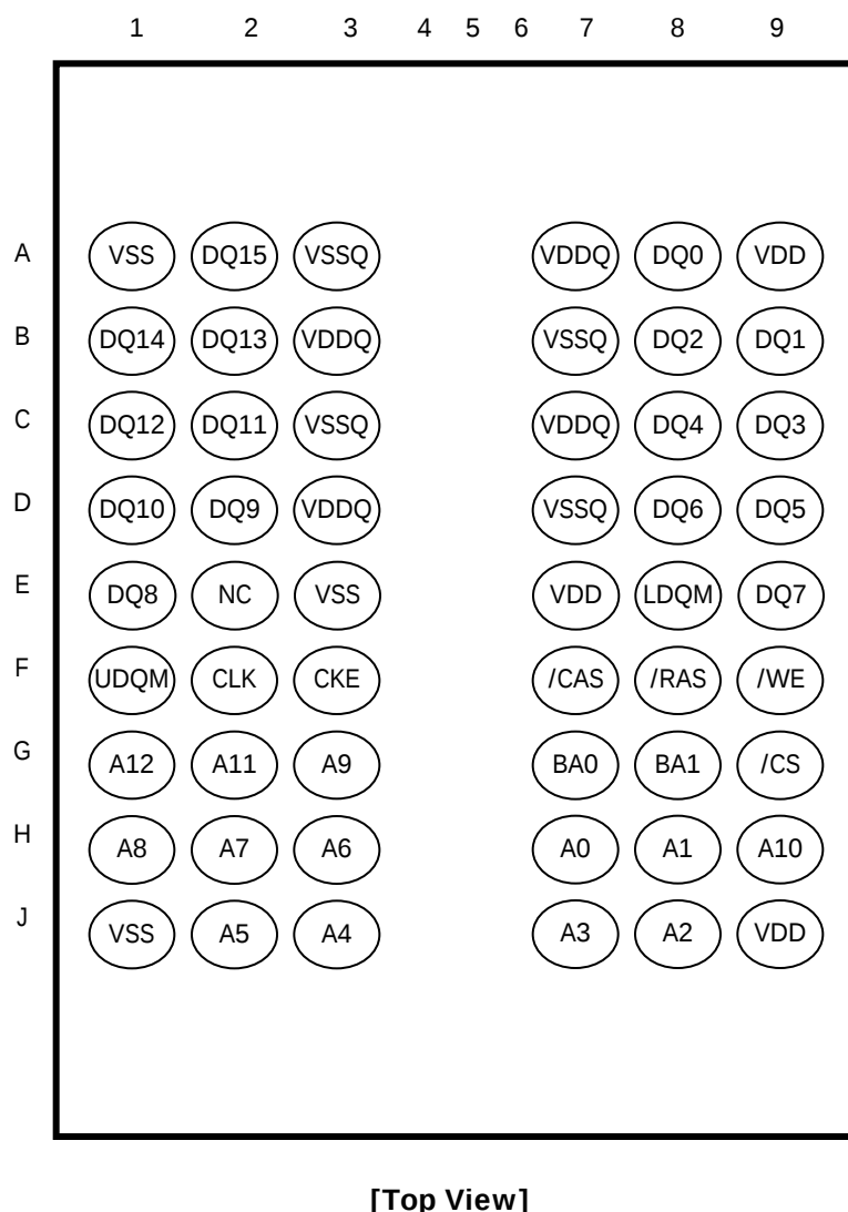
Figure1: 54Ball FBGA Ball Assignment
