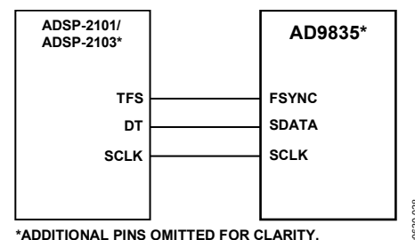
Figure 26. ADSP-2101/ADSP-2103 to AD9835 Interface
