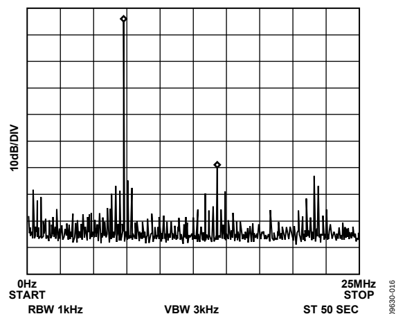
Figure 16. f_{MCLK} = 50 MHz, f_{OUT} = 7.1 MHz. Frequency Word = 245A1CAC
