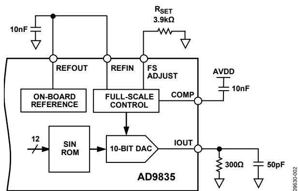
Figure 2. Test Circuit
