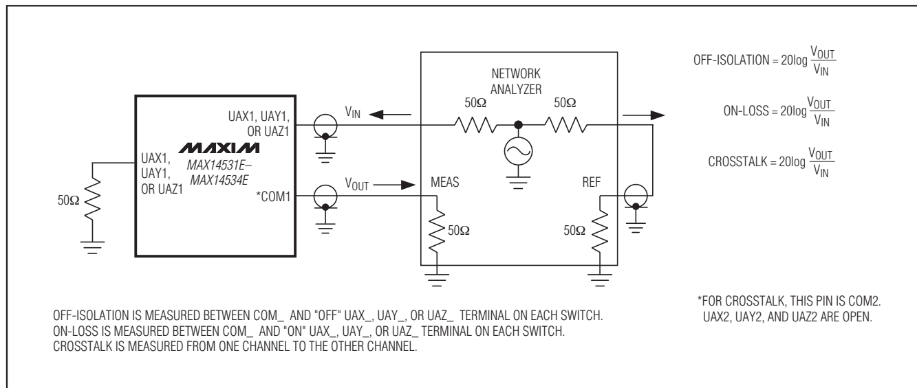
Figure 3. On-Loss, Off-Isolation, and Crosstalk
