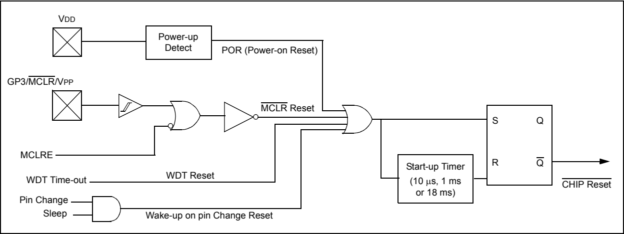
FIGURE 8-8: TIME-OUT SEQUENCE ON POWER-UP ( \overline{\text{MCLR}} PULLED LOW)
