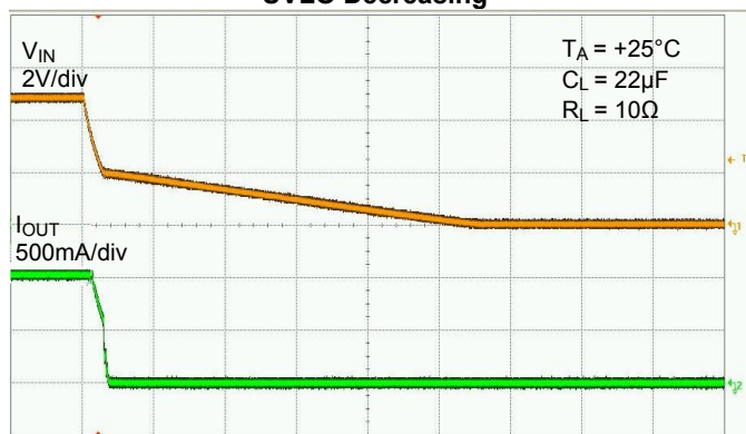
UVLO Decreasing
