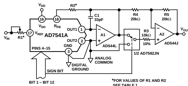
Figure 6. 12-Bit Plus Sign Magnitude Operation
