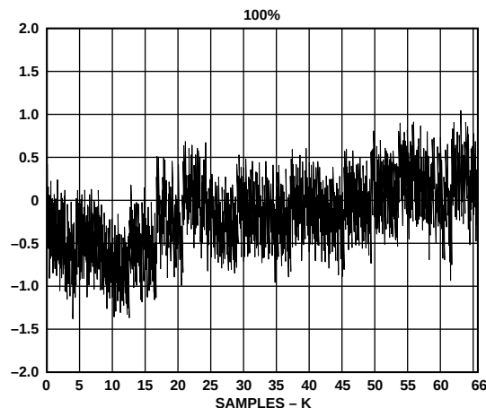
Figure 17. INL Plot
