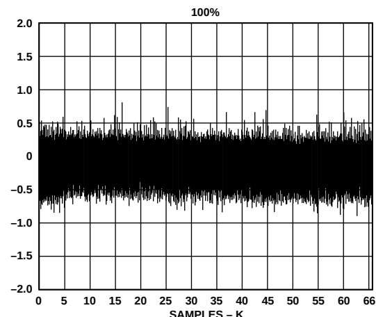
Figure 18. DNL Plot
