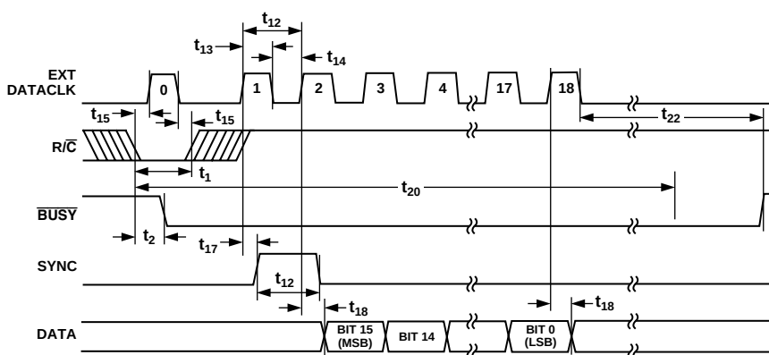
Figure 7. Conversion and Read Timing for Reading Previous Conversion Results During a Conversion Using External Discontinuous Data Clock (EXT/ \overline{INT} Set to Logic High, \overline{CS} Set to Logic Low)
