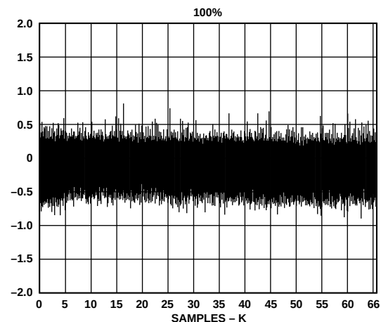
Figure 18. DNL Plot
