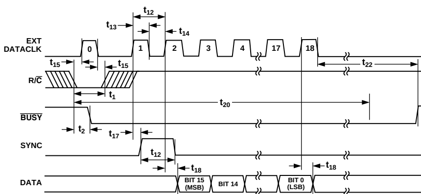
Figure 7. Conversion and Read Timing for Reading Previous Conversion Results During a Conversion Using External Discontinuous Data Clock (EXT/INT Set to Logic High, \overline{CS} Set to Logic Low)
