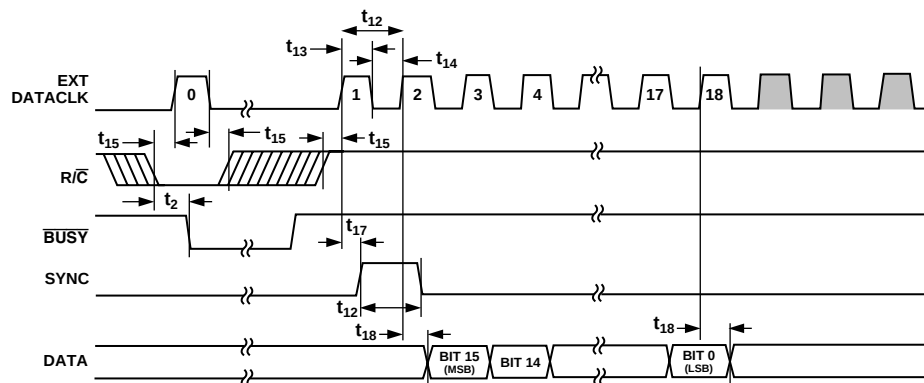
Figure 6. Conversion and Read Timing Using An External Discontinuous Data Clock (EXT/INT Set to Logic High, \overline{\text{CS}} Set to Logic Low)
