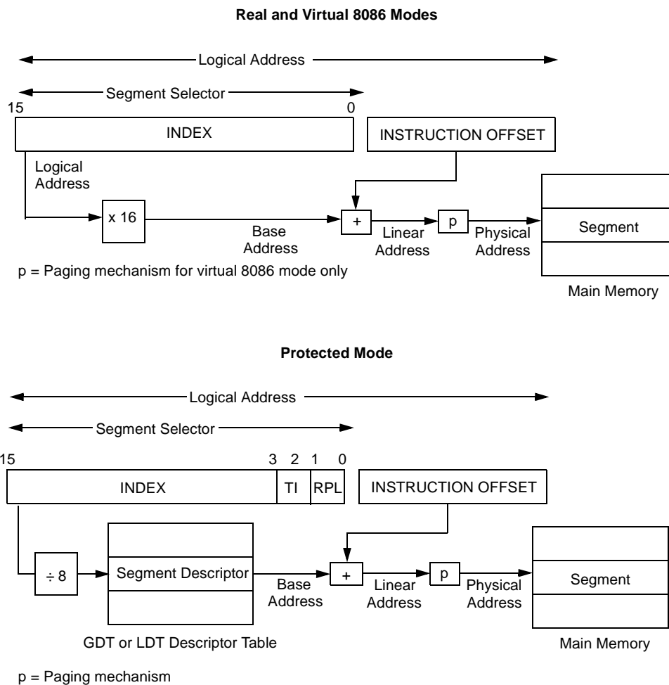
Figure 3-6. Selector Mechanisms
