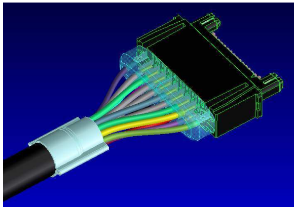
Figure 9. Crimp barrel installed
