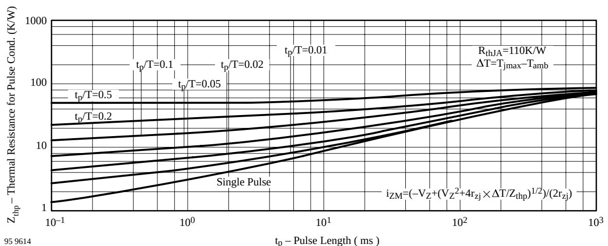
Figure 5. Thermal Response
