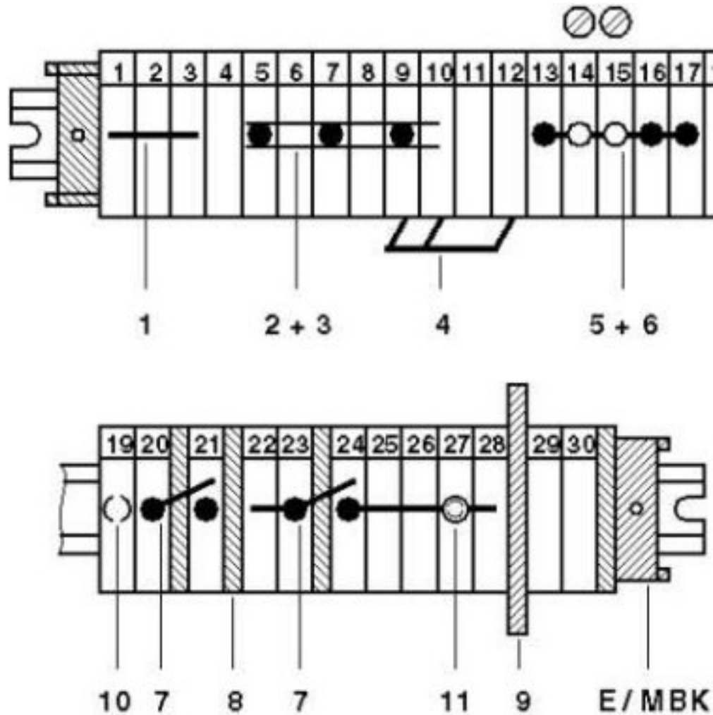
Circuit diagram
