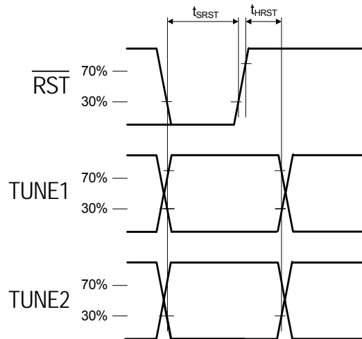
Figure 1. Reset Timing
