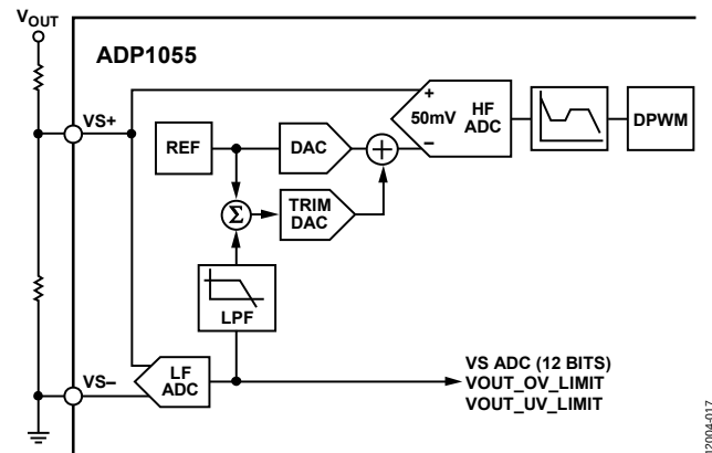
Figure 22. Output Voltage Sense and Feedback
