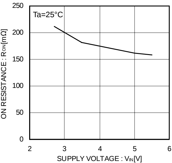
Figure 10. On-resistance
