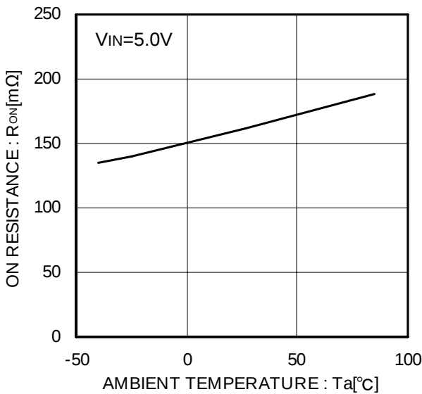
Figure 11. On-resistance
