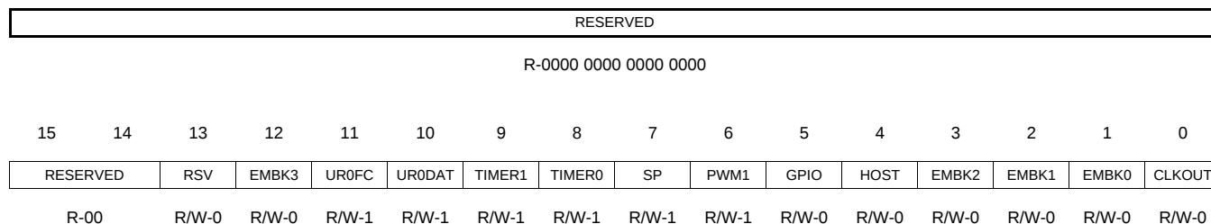
Figure 3-1. VDD3P3V_PWDN Register
