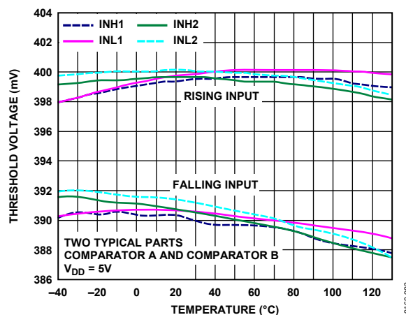
Figure 2. Comparator Thresholds vs. Temperature
