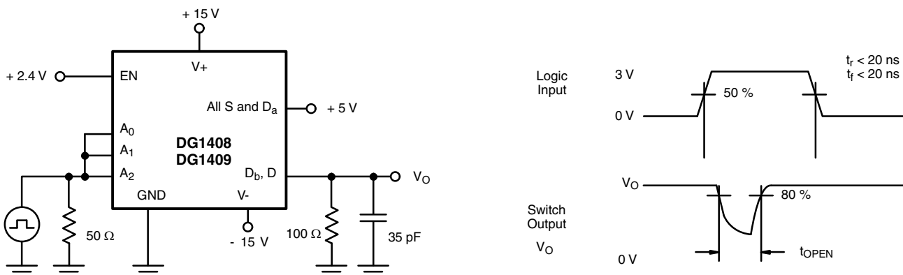
Fig. 3 - Break-Before-Make Internal
