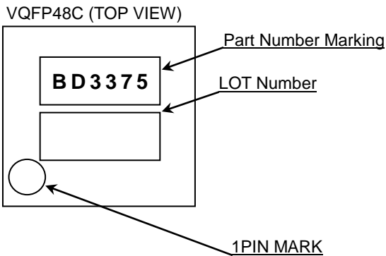
Figure 125. Marking Diagrams
