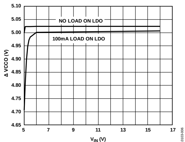
Figure 6. V_{CCO} Line Regulation
