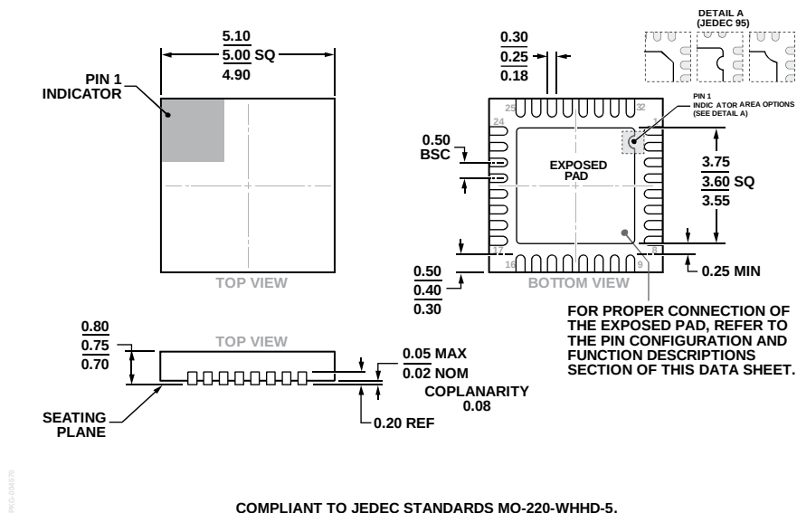
COMPLIANT TO JEDEC STANDARDS MO-220-WHHD-5. Figure 34. 32-Lead Lead Frame Chip Scale Package [LFCSP] 5 mm × 5 mm Body, and 0.75 mm Package Height (CP-32-12) Dimensions shown in millimeters
