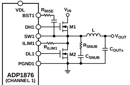
Figure 32. Application Circuit with a Snubber
