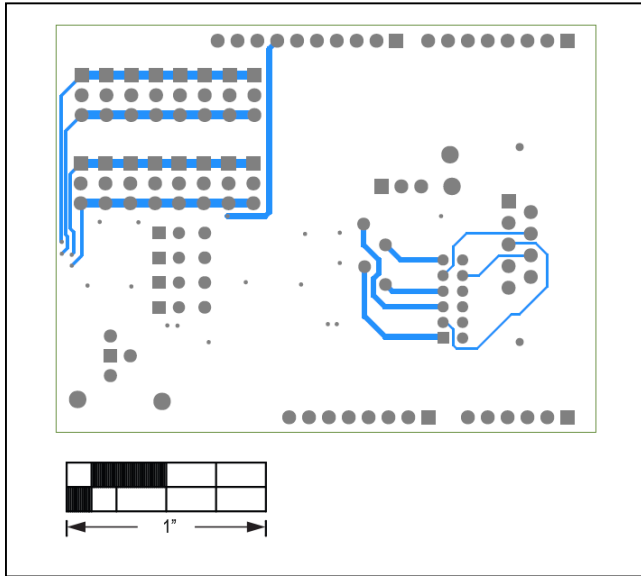
MAX33250E Shield—Bottom
