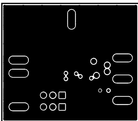
Figure 38. Bottom Layer
