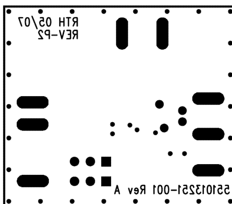
Figure 39. Bottom Silkscreen
