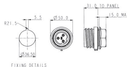
FIXING DETAILS
