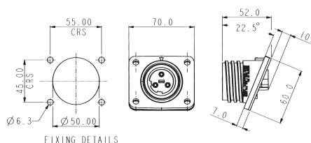
FIXING DETAILS
