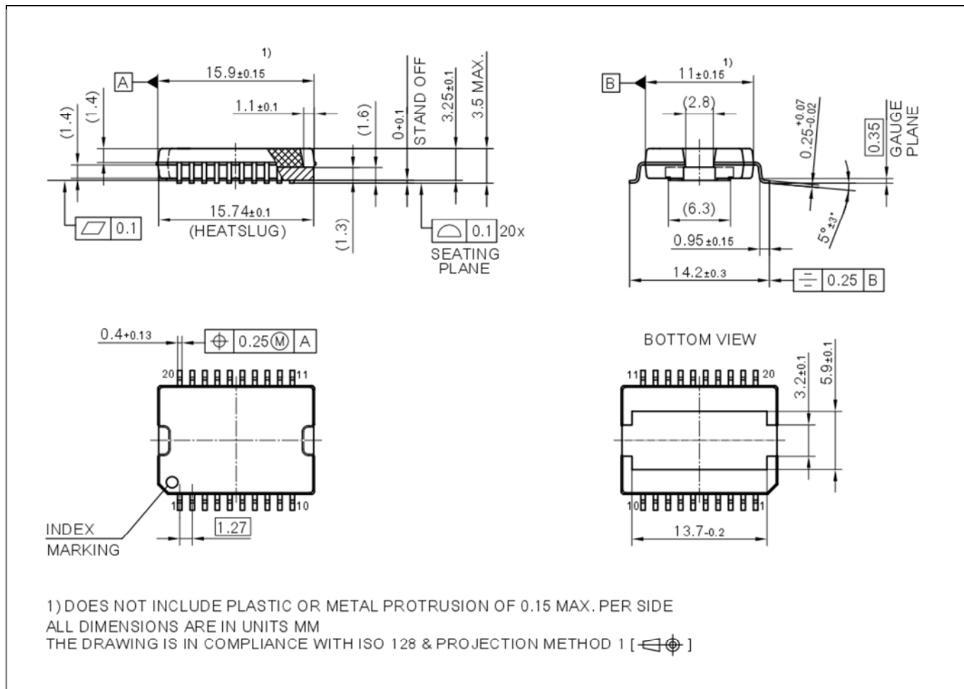
Figure 28 PG-DSO-20-85 Package Outline, dimensions (mm)
