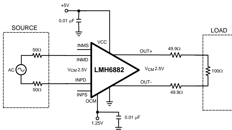
Figure 42. Typical Implementation with a Differential Input Signal
