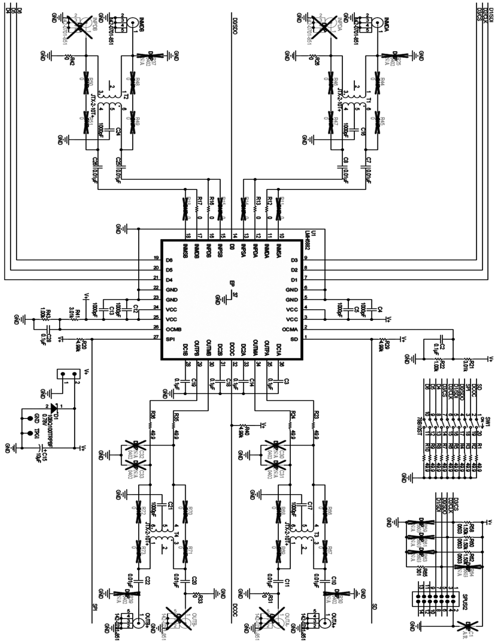
Figure 53. Evaluation Board Schematic
