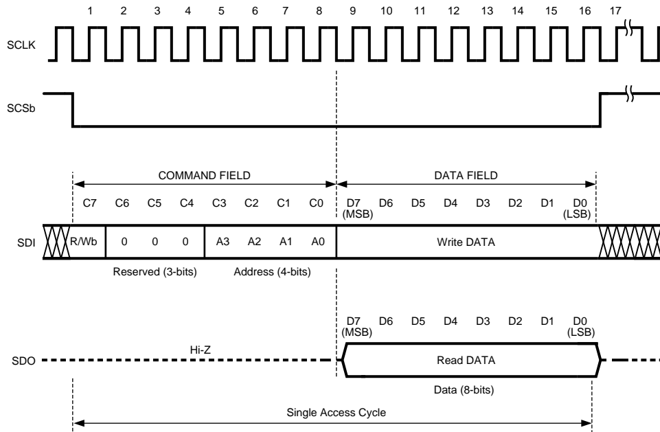
Figure 50. Serial Interface Protocol (SPI compatible)
