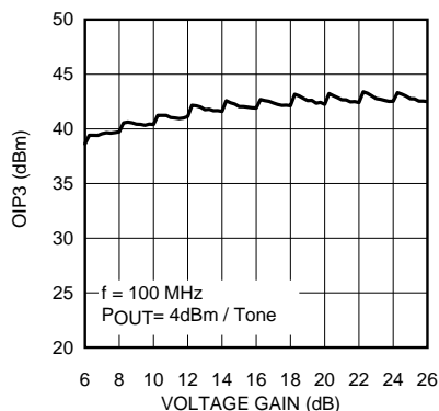
Figure 1. OIP3 over Voltage Gain Range
