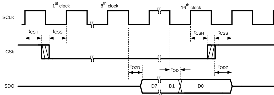
Figure 52. Read Timing
