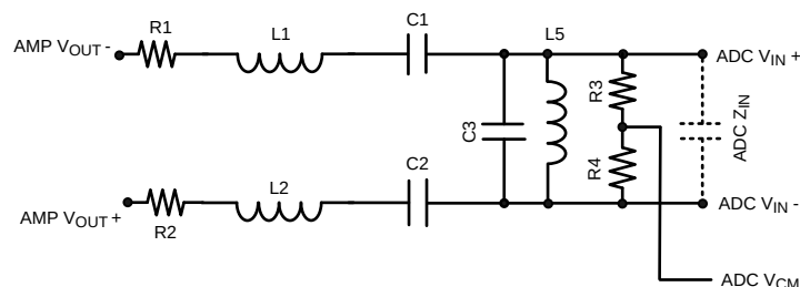
Figure 46. Sample Filter
