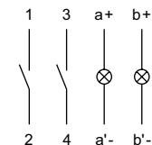
Wiring diagram 10
