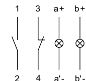
Wiring diagram 13
