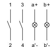
Wiring diagram 9
