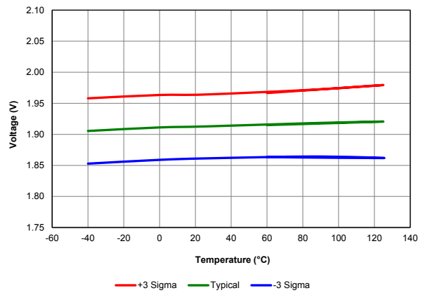
Figure 39-20. Brown-Out Reset Voltage, Trip Point (BORV = 11) for PIC18LF24/25K40 only
