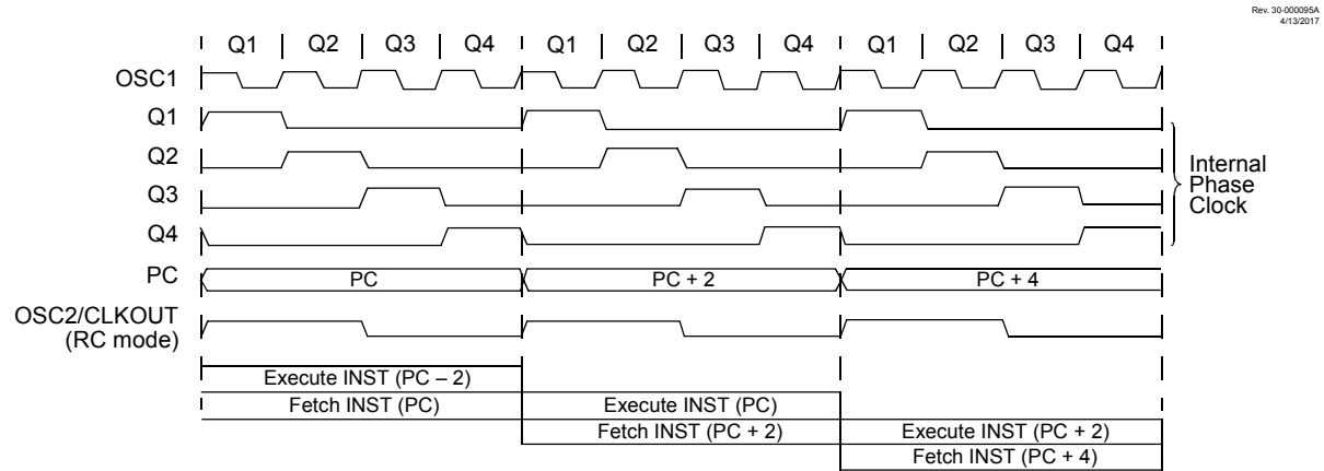
Figure 10-4. CLOCK/INSTRUCTION CYCLE
