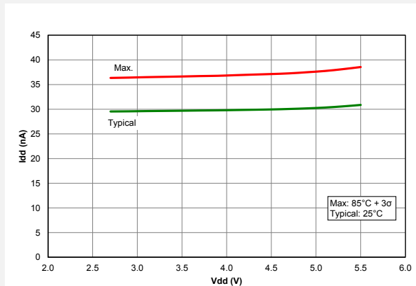
Figure 39-64. I_{DD} , Fixed Voltage Reference (FVR), PIC18F24/25K40 only
