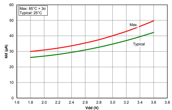
Figure 39-65. I_{DD} , Brown-out Reset, BORV = 1, PIC18LF24/25K40 only
