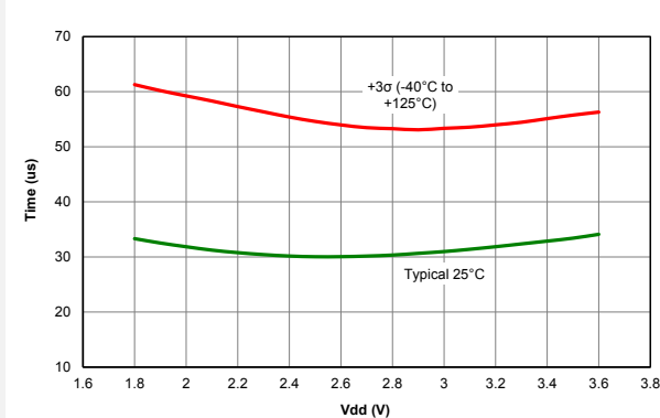
Figure 39-11. Bandgap Ready Time, PIC18LF24/25K40
