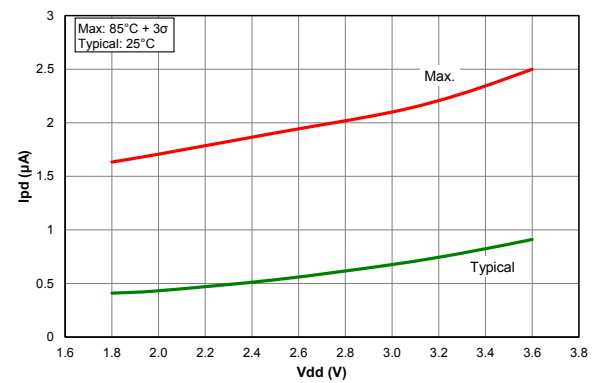
Figure 39-63. I PD , Fixed Voltage Reference (FVR), PIC18LF24/25K40 only
