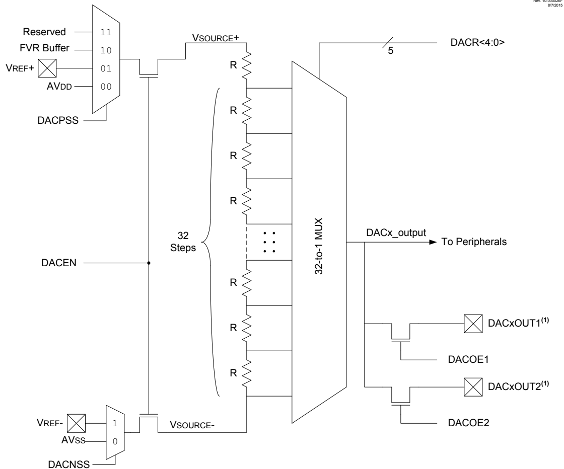
Figure 30-1. Digital-to-Analog Converter Block Diagram
