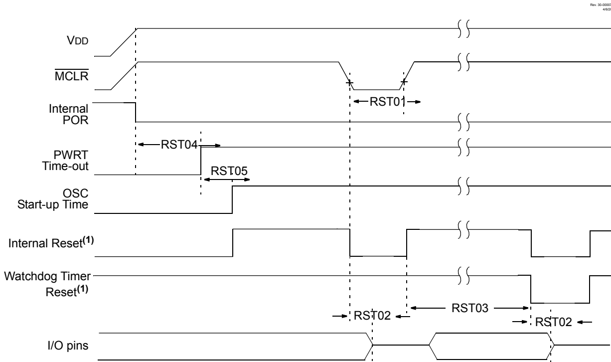
Figure 38-8. Reset, Watchdog Timer, Oscillator Start-up Time and Power-up Timer Timing
