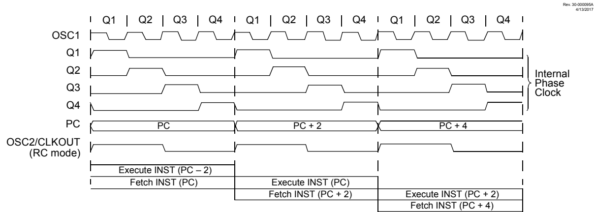
Figure 10-4. CLOCK/INSTRUCTION CYCLE
