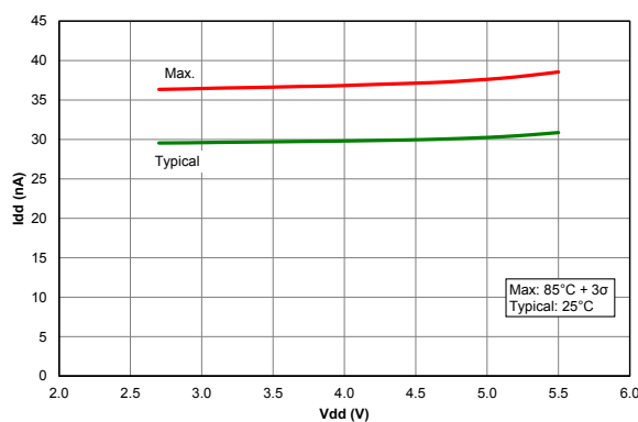
Figure 39-64. I_{PD} , Fixed Voltage Reference (FVR), PIC18F24/25K40 only
