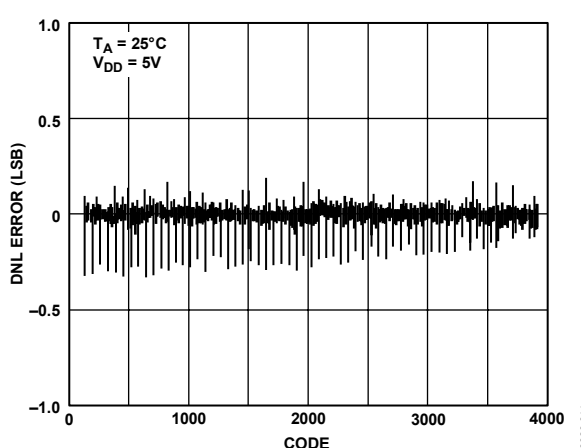
Figure 9. AD5325 Typical DNL Plot
