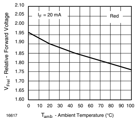
Figure 8. Forward Voltage vs. Ambient Temperature
