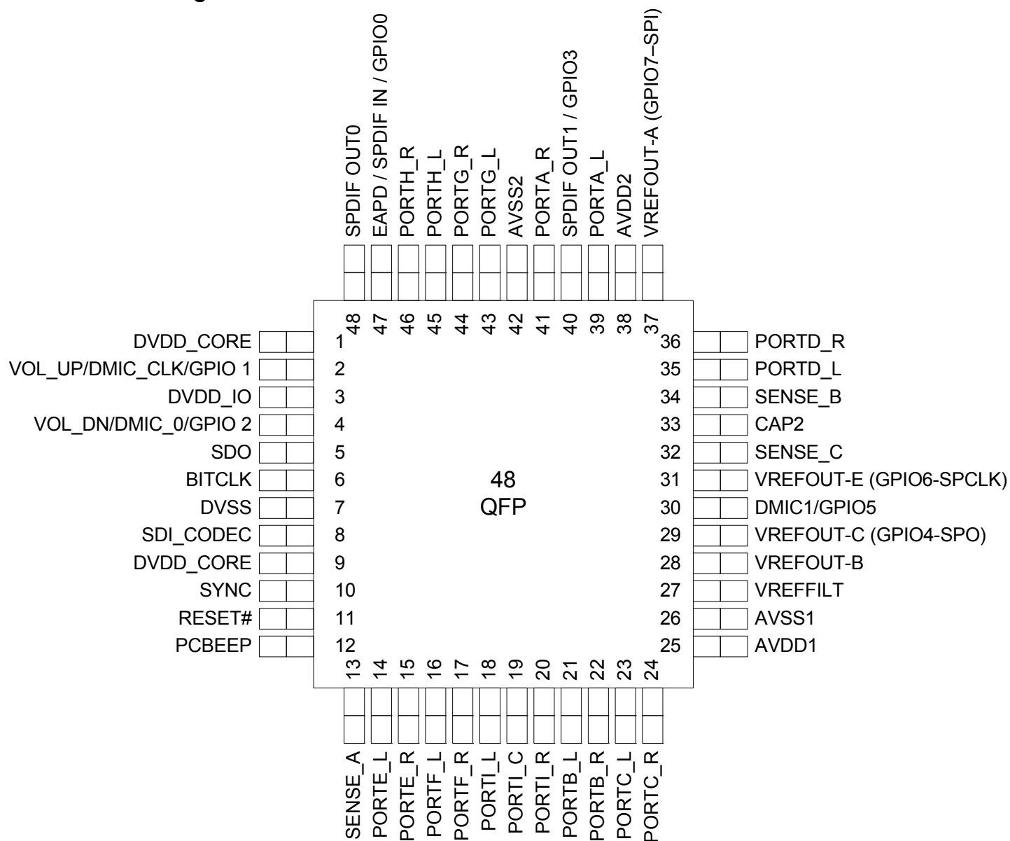
Figure 13. Pin Assignment
