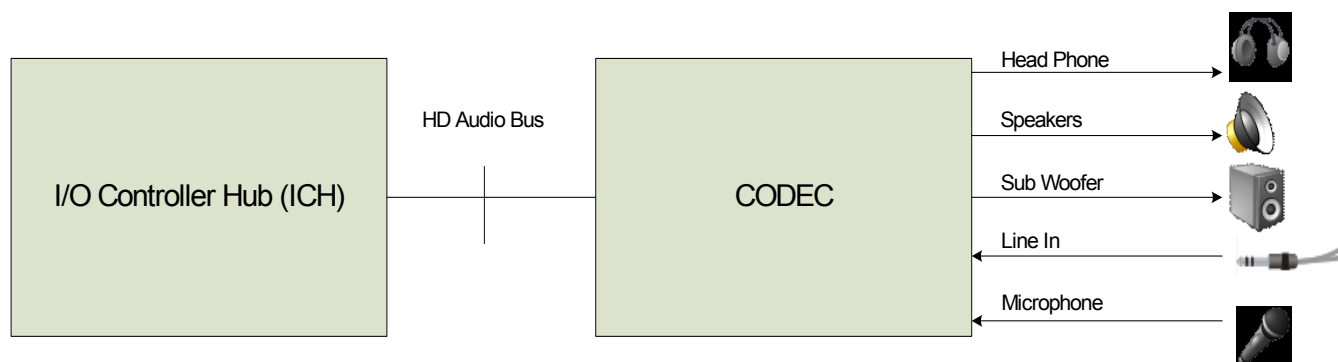
Figure 2. System Diagram
