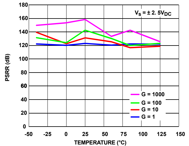
FIGURE 22. PGIA PSRR vs TEMPERATURE
