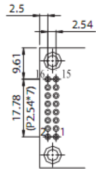
PIN DETAIL
