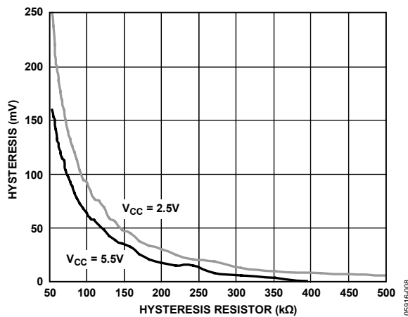
Figure 10. Hysteresis vs. Hysteresis Resistor
