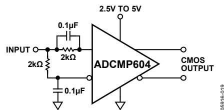
Figure 21. Self-Biased, 50% Slicer
